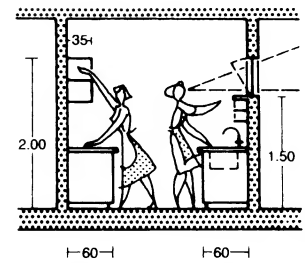
4 Worktops and storage 60cm deep
